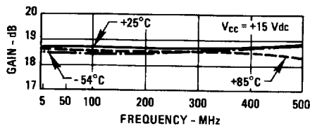
Gain
