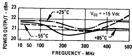
Power Output*
