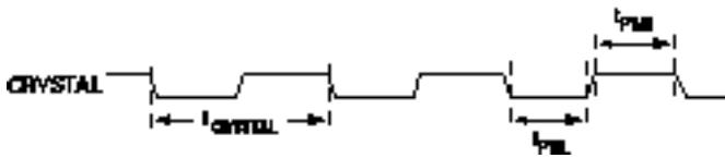
Figure 26. Clock Timing
