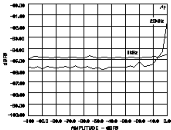
Figure 19. THD+N vs. Input Amplitude, 44.1 kHz Input Sample Frequency, 48 kHz Output Sample Frequency, 1 kHz and 20 kHz Tones
