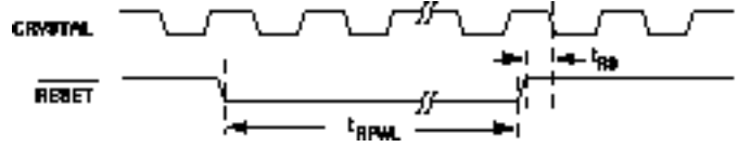
Figure 27. Reset Timing
