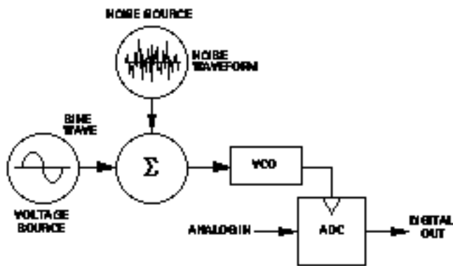
Figure 7. Clock Jitter Modeled as a Modulated VCO
