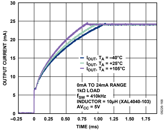
Figure 50. Output Current Settling with DC-to-DC Converter vs. Time and Temperature (See Figure 80)
