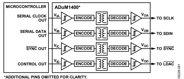
Figure 88. Isolated Interface
