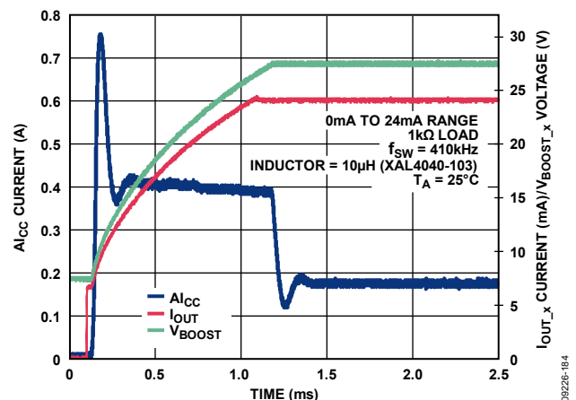
Figure 82. A_{\text{ICC}} Current vs. Time for 24 mA Slew with Internal Compensation Resistor
