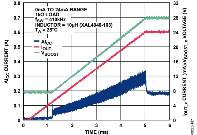
Figure 85. I_{CC} Current vs. Time for 24 mA Slew with Slew Rate Control
