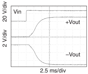
80% load each output MOR2805D Turn On Response FIGURE 47
