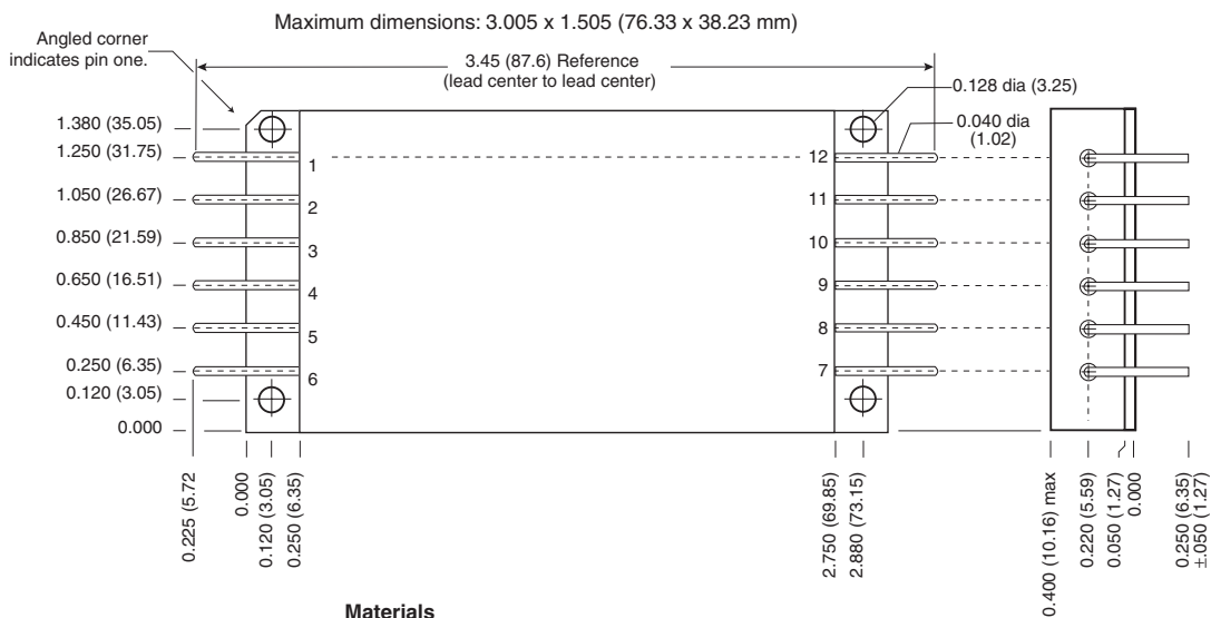
PIN-SIDE VIEW CASE V* Flanged case, down leaded) *Requires case option designator added to model number: MOR2805SV
