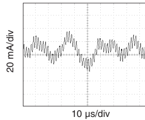
MOR2815S Input Ripple (lin) FIGURE 37
