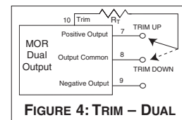
FIGURE 4: TRIM - DUAL
