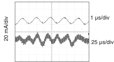
MOR2812D Input Ripple (Iin) FIGURE 49
