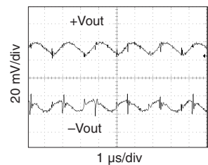
80% load each output MOR2805D Output Ripple (±Vout) FIGURE 41
