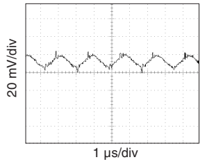
MOR2805S Output Ripple (Vout) FIGURE 30
