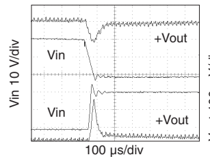
18 to 40 V, 40 to 18 V MOR2812D Step Line Response FIGURE 52
