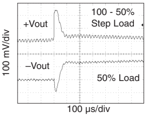
MOR2812D Step Load Response FIGURE 50
