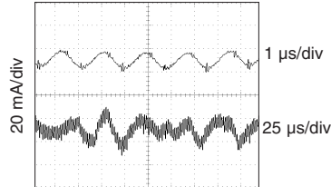
MOR2805S Input Ripple Current (Iin) FIGURE 31
