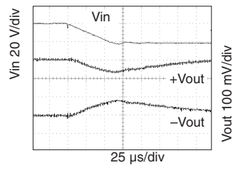
40 to 18 V, 80% load each output MOR2805D Step Line Response FIGURE 46
