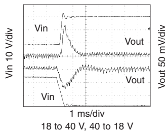
MOR2805S Step Line Response FIGURE 33
