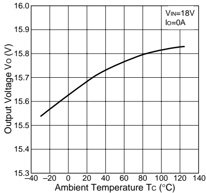
Temperature Coefficient of Output Voltage(SI-3157B)
