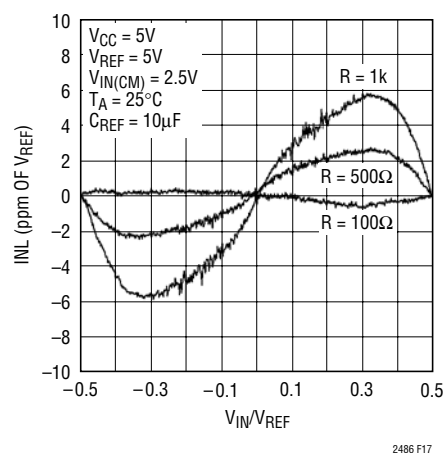
Figure 17. INL vs Differential Input Voltage and Reference Source Resistance for C_{REF} > 1\text{ }\mu\text{F}
