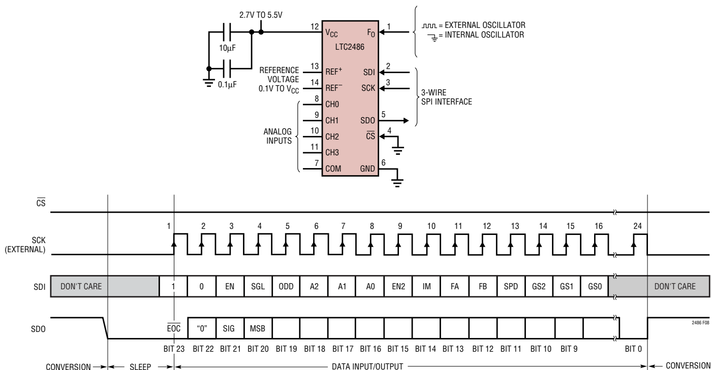
Figure 8. External Serial Clock, 3-Wire Operation (CS = 0)
