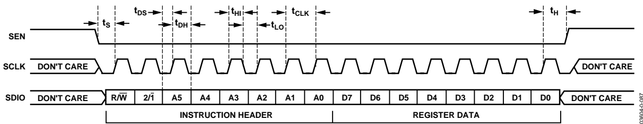
Figure 52. 1-Byte Serial Register Write in MSB First Mode
