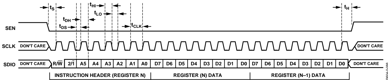
Figure 53. 2-Byte Serial Register Write in MSB First Mode
