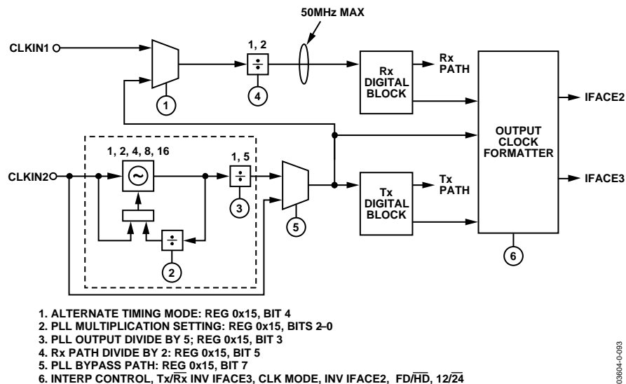
Figure 58. Clock Distribution Block Diagram
