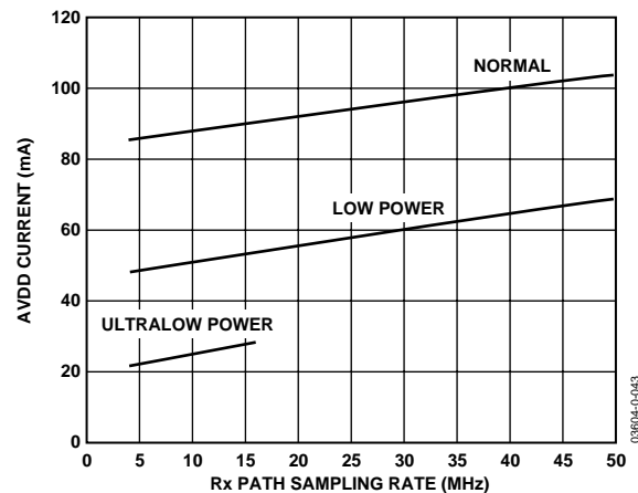
Figure 49. Typical Rx Path Analog Supply Current vs. Sample Rate, V_{DD} = 3.3 \text{ V} for Normal, Low and Ultralow Power Modes
