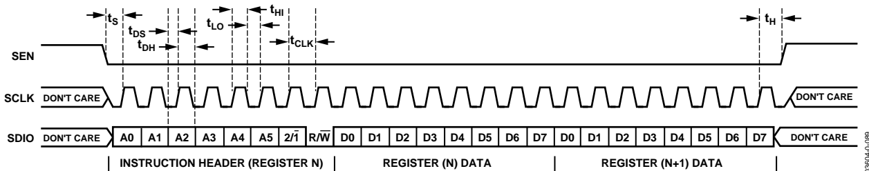
Figure 54. 2-Byte Serial Register Write in LSB First Mode
