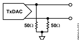
Figure 2. Diagram showing Termination of 100\ \Omega Differential Load for Some TxDAC Measurements
