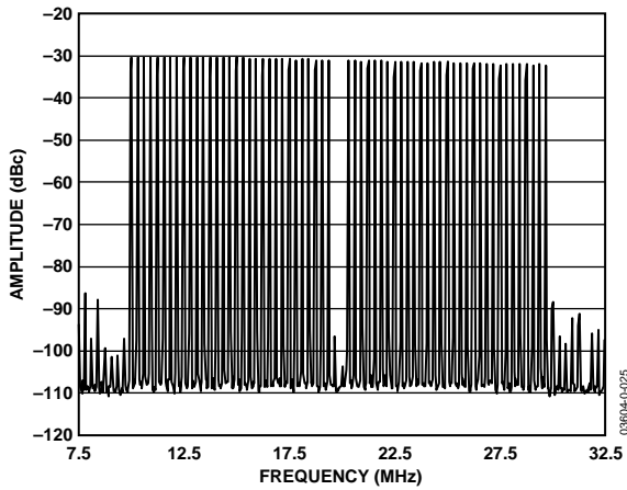
Figure 28. AD9863 Tx Path FFT, 64-Carrier (Center Two Carriers Removed) OFDM Signal over 20 MHz Bandwidth, Centered at 20 MHz, with 20 mA Full-Scale Output into 60 \Omega Differential Load
