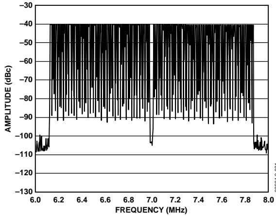
Figure 34. AD9863 Tx Path FFT, 256-Carrier (Center Four Carriers Removed) OFDM Signal over 1.75 MHz Bandwidth, Centered at 7 MHz, with 20 mA Full-Scale Output into 60 Ω Differential Load
