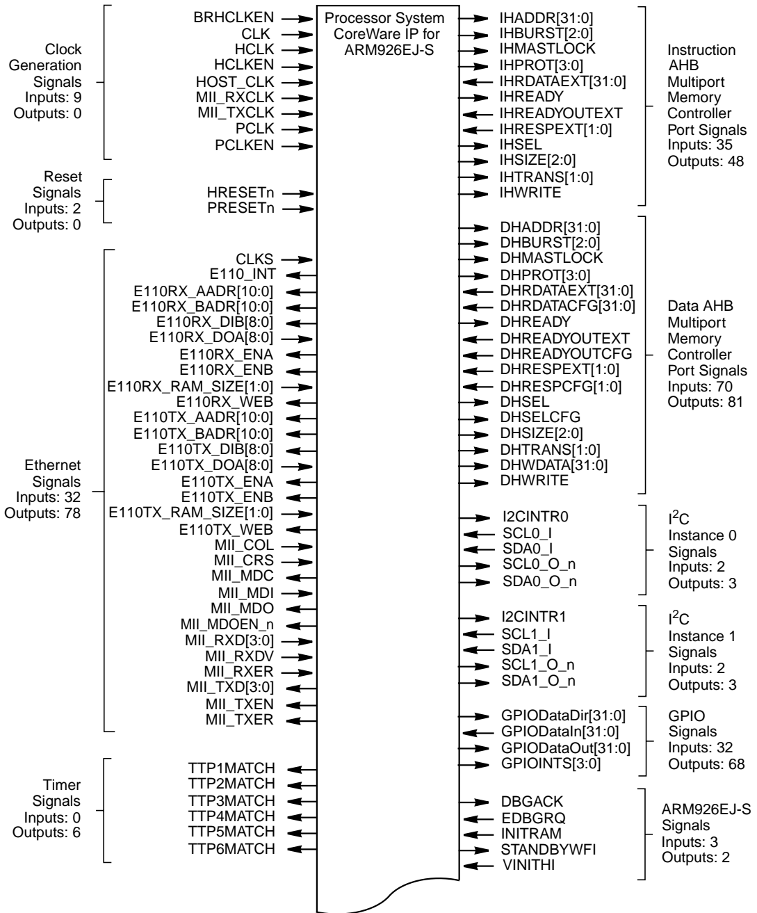
Figure 4.1 System Interfaces
