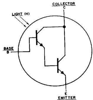
PHOTO-DARLINGTON CIRCUIT
