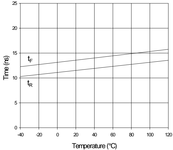
Fig. 5 Rise And Fall Times vs. Temperature C_L = 18 \text{ V} V_{CC} = 18 \text{ V}
