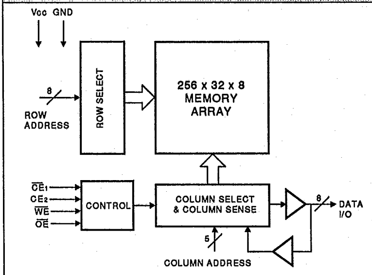
L7C185/L7CL185 Block Diagram
