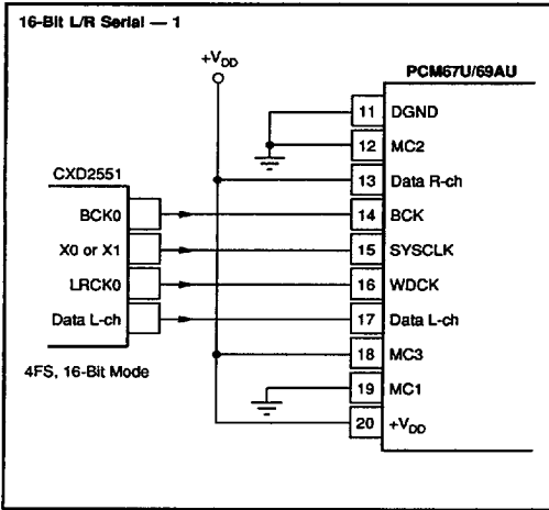
FIGURE 8. Using Sony CXD2551.
