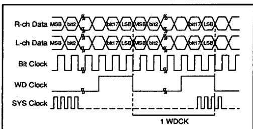
FIGURE 3. Timing Diagram.
