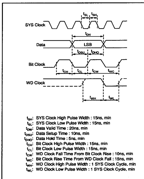
FIGURE 4. Timing Specification.
