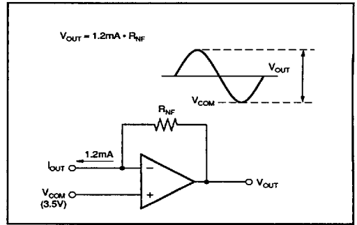
FIGURE 2. I/V Amplifier Circuit.
