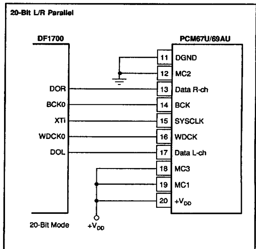
FIGURE 11. Using Burr-Brown DF1700.
