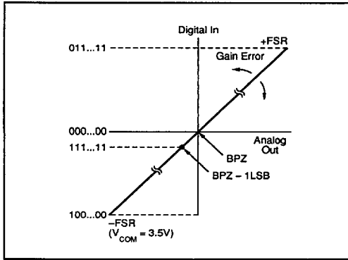
FIGURE 1. Transfer Performance.
