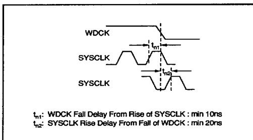
FIGURE 5. Timing of PCM69A for SYSCLOCK and WDCK.
