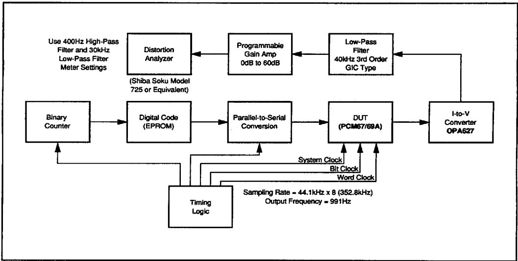
FIGURE 12. PCM67/69A THD + N Production Test.
