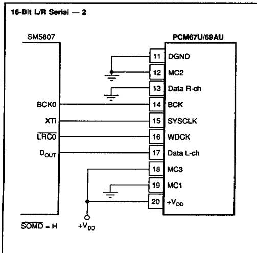
FIGURE 9. Using NPC SM5807.
