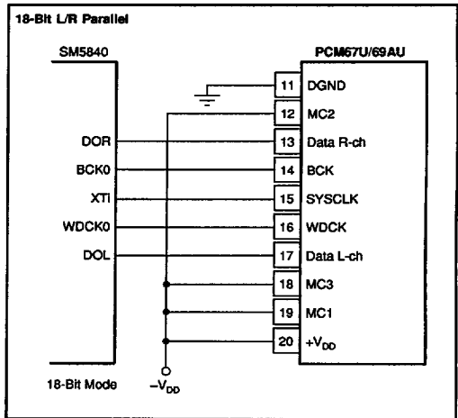
FIGURE 10. Using NPC SM5840.
