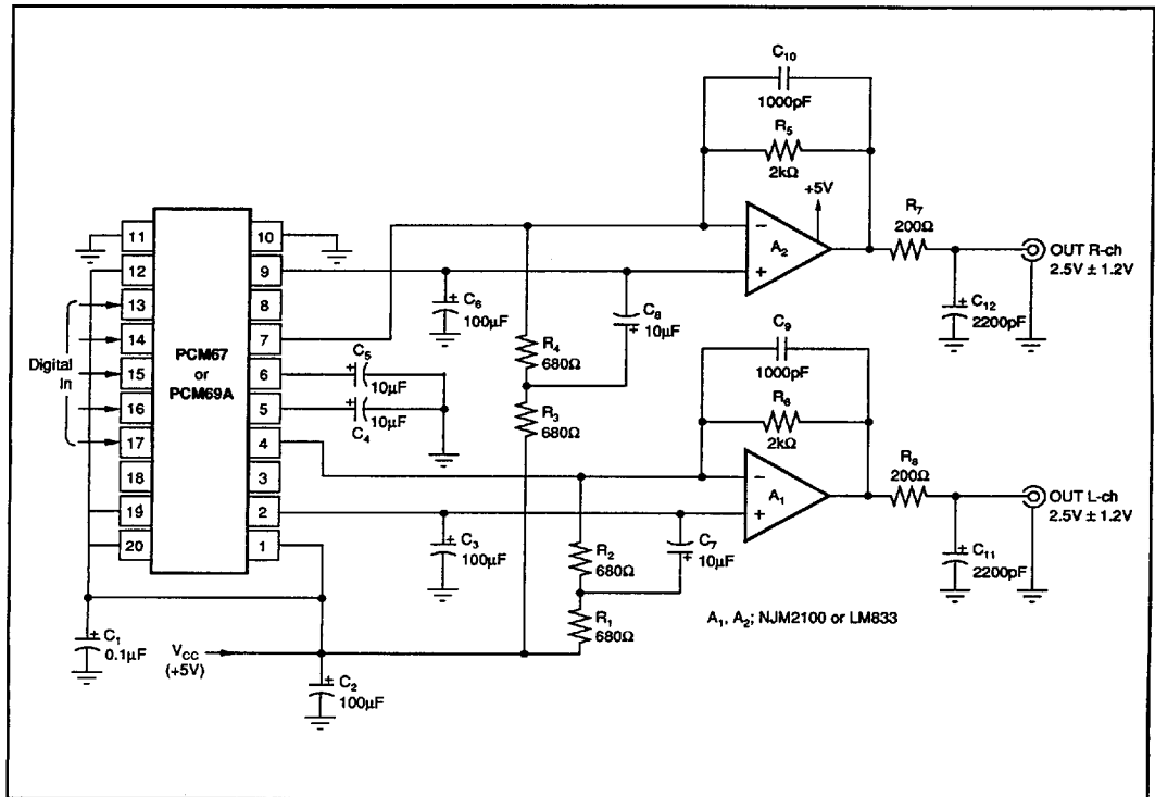
FIGURE 13. Single +5V Power Supply, with LPF, I/V Amp Application Circuit for Portable Digital Audio.
