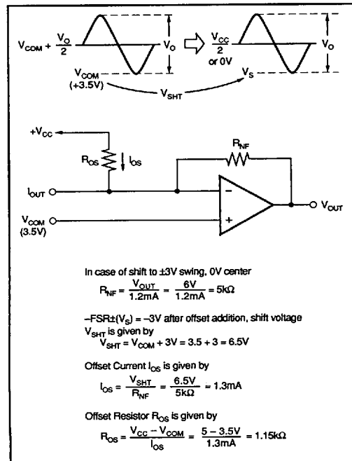
FIGURE 6. Shift of I/V Out Voltage.
