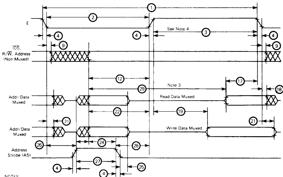
FIGURE 6 — BUS TIMING
