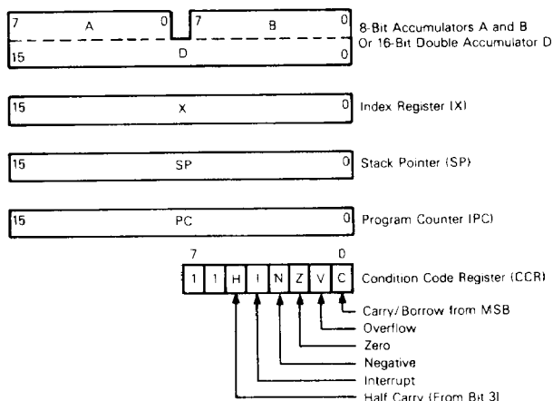
FIGURE 9 — PROGRAMMING MODEL
