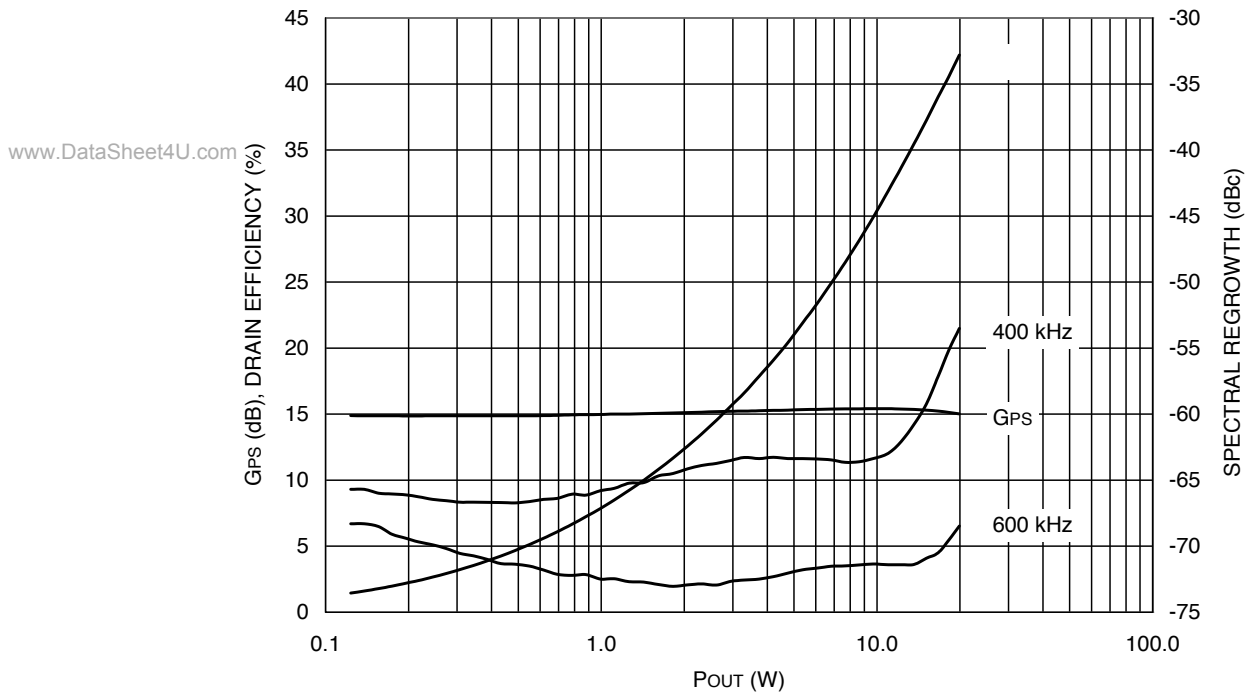
Figure 9. Power Gain, Efficiency, and Spectral Regrowth vs. Output Power
