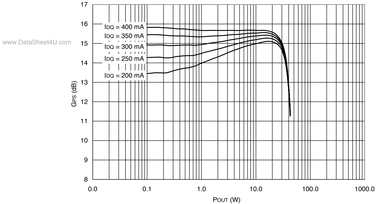
Figure 5. CW Power Gain vs. Output Power
