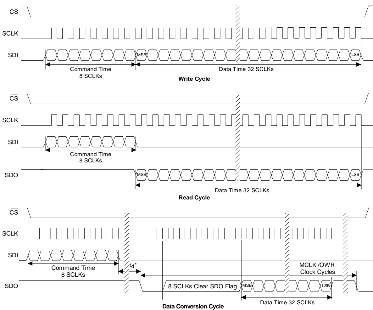
Figure 7. Command and Data Word Timing.
