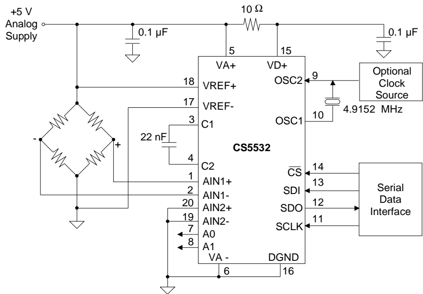
Figure 16. CS5532 Configured with a Single +5 V Supply.
