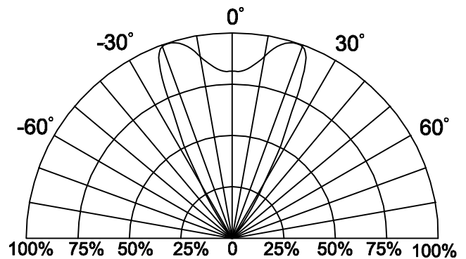
Fig.6 Directivity Radiation
