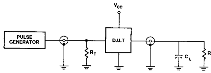
Test Circuit
