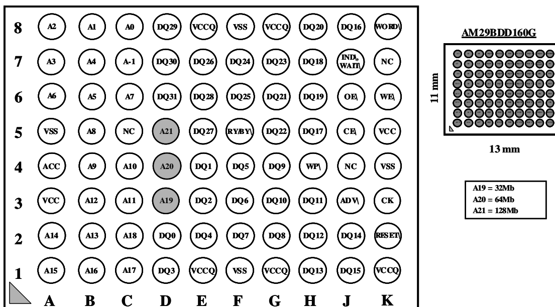
Figure 3-3. 80-Ball Fortified-BGA
