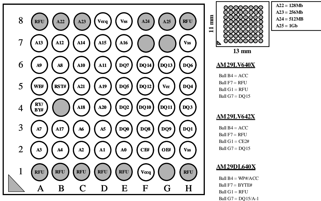
Figure 3-2. 64-Ball Fortified-BGA
