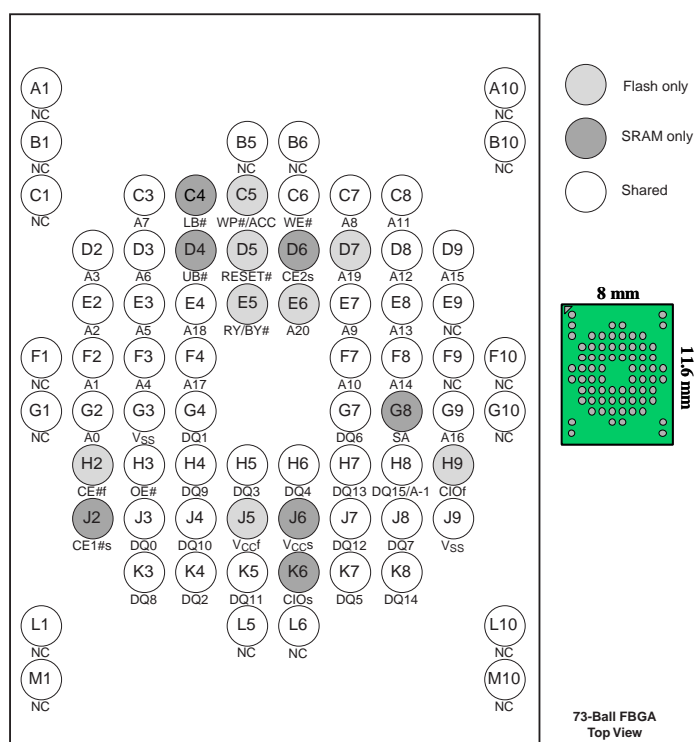
Figure 4-7. Am29DL32XD and 8Mb (x8/x16) SRAM MCP Pinout
