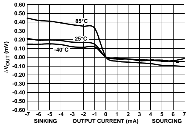
FIGURE 22. LOAD REGULATION
