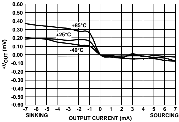
FIGURE 91. LOAD REGULATION I_{SOURCE}-I_{SINK} = \pm 7mA
