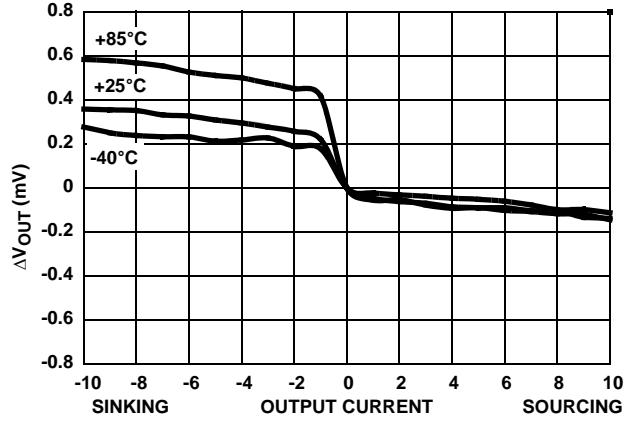
FIGURE 49. LOAD REGULATION
