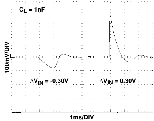
FIGURE 34. LINE TRANSIENT RESPONSE
