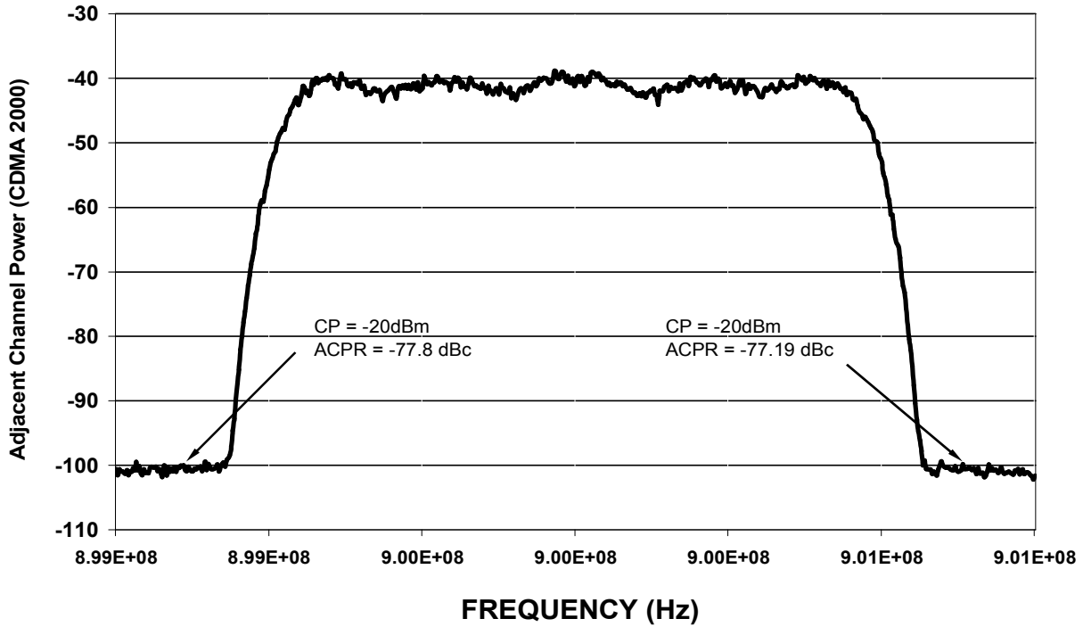
CDMA 2000 @ 900 MHz, ACPR @ 885 kHz, VCC = 5V
