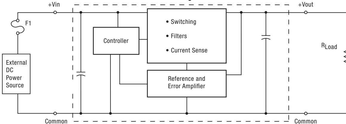
Figure 1. OKI-78SR
