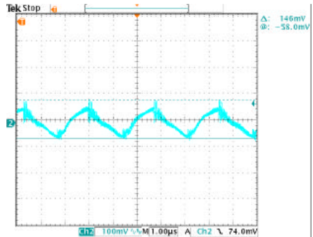
Figure 22. Output voltage Ripple & Noise, at Vin=48v, Iout=20A, with 10uF tantalum cap. and 1uf ceramic cap. output capacitance load.
