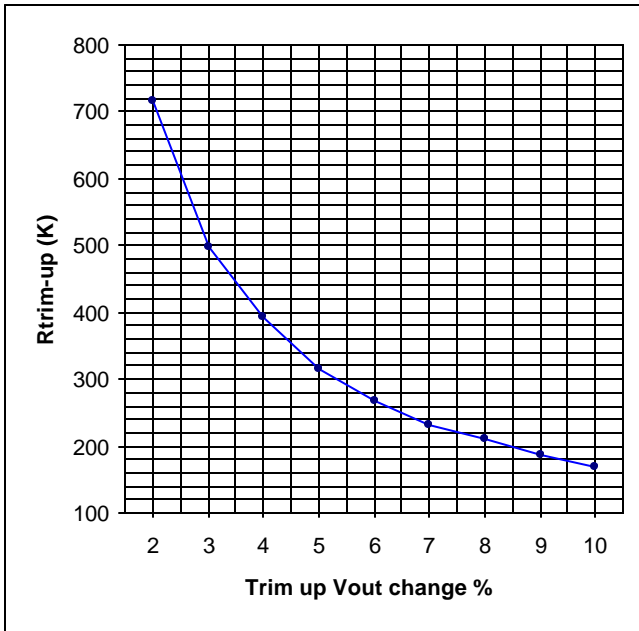
Fig 5. Trim Up Resistance for reference chart
