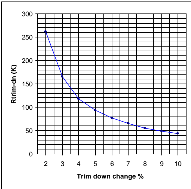
Fig 6 Trim Down Resistance for reference chart
