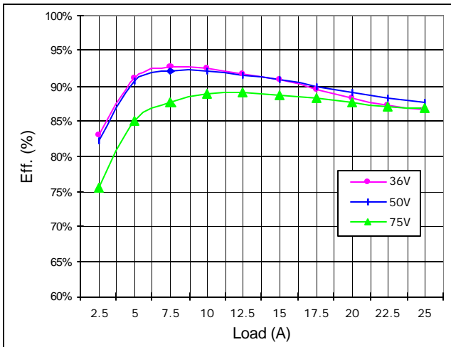
Figure 14. Efficiency at nominal output voltage vs. output current for various Input voltage. The unit mounted on the 0.06" thick PCB with 300LFM air flow (1.5/m) from pin 3 to pin 4 and Ta=25°C
