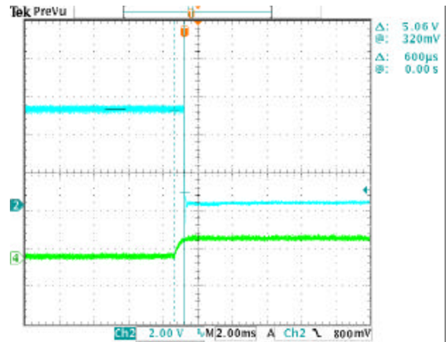
Figure 13. Turn off timing vs. Input On/Off Pin. Waveform 2 is output voltage, waveform 4 is negative On/Off logic signal. At 48v input voltage, 20A output current with 100uf output capacitance load.
