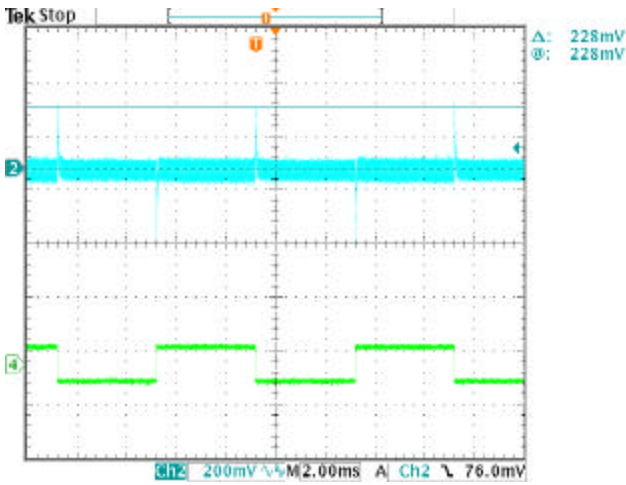
Figure 15. Output voltage dynamic response at Vin=48v Iout= 12~20A, 2.5A/us dynamic load. waveform 2 is dynamic response via dynamic load. waveform 4 is load current (2.5A/us); with 10uF output capacitance load.
