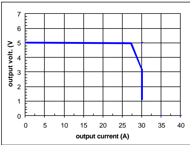
Figure 19. Output voltage vs. output current limit point and the unit shutdown point. Input voltage has almost no effect on current limit point.
