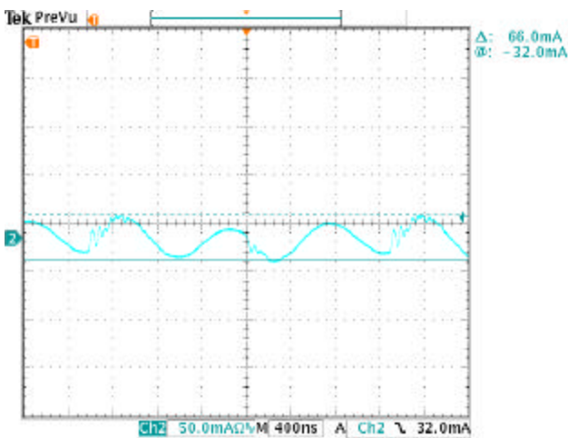
Figure 26. Input reflected ripple current \dot{I}_c waveform without input inductor. At V_{in}=48v , I_{out}=25A , 50ma/Div. ( current probe with 50mv/div )
