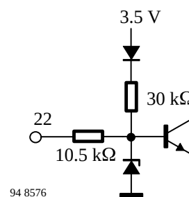
Figure 18. AFC control switch (Pin 22)
