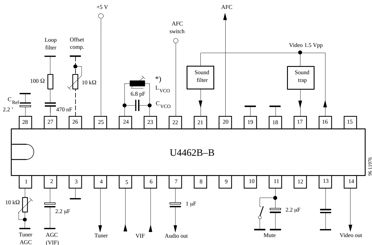
Figure 3. Test circuit
