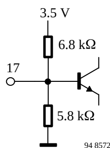
Figure 14. Video input (6 dB amplifier) (Pin 17)
