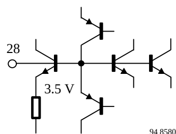
Figure 22. Internal reference voltage (Pin 28)
