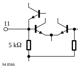
Figure 11. Decoupling capacitor (Pin 11) and mute switch
