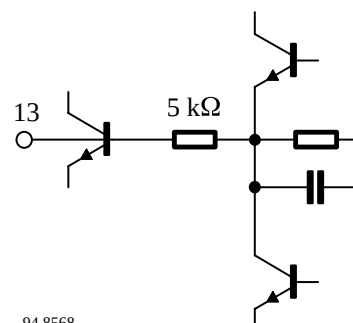
Figure 12. De-emphasis (Pin 13)
