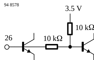
Figure 20. Offset compensation (Pin 26)
