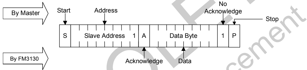
Figure 9. Current Address Memory Read
