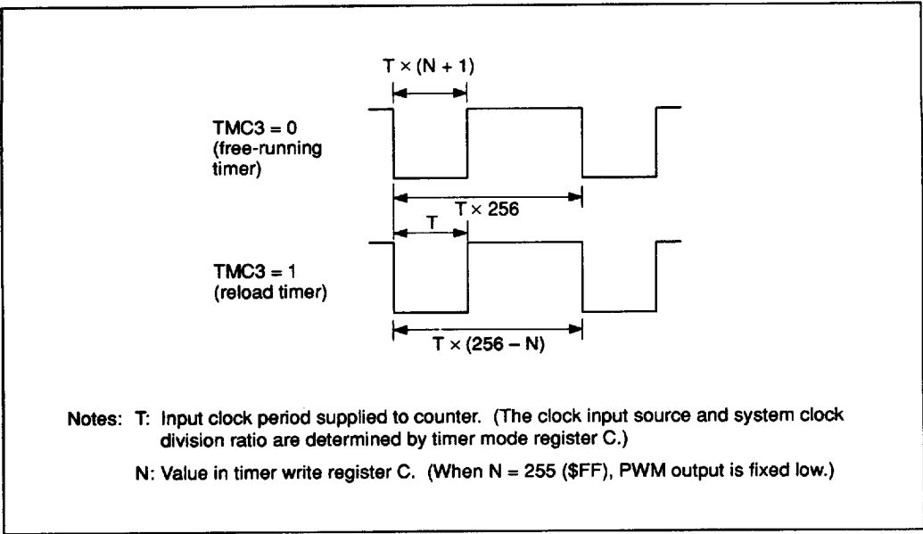
Figure 35 PWM Output Waveform
