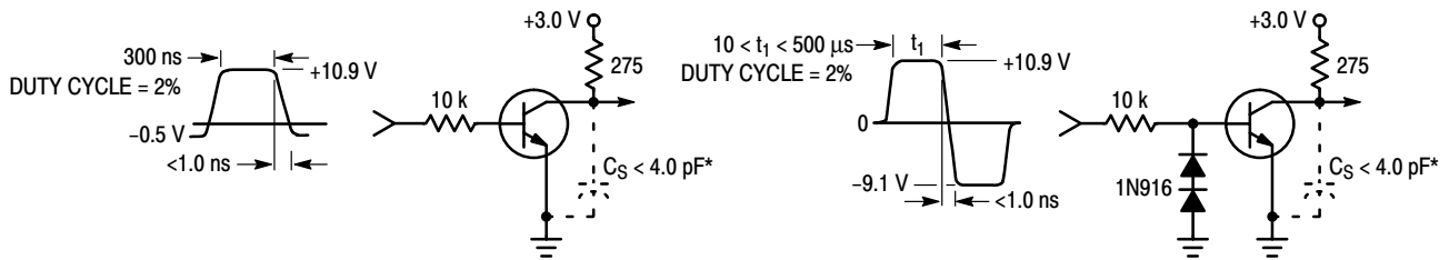
Figure 1. Turn–On Time
