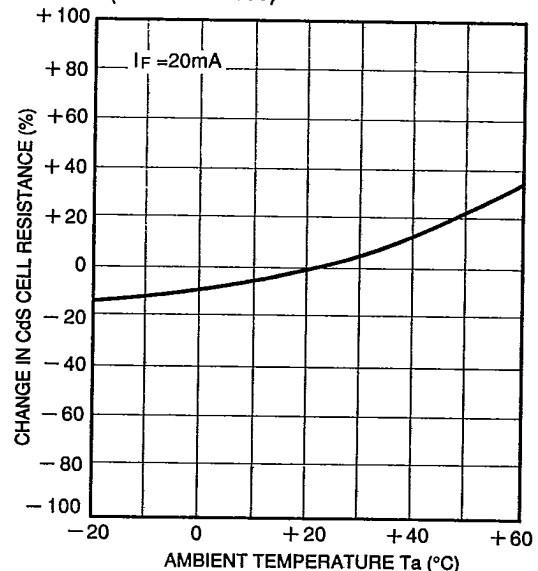
Figure 7: Output Resistance vs. Temperature (P873-G35-380)
