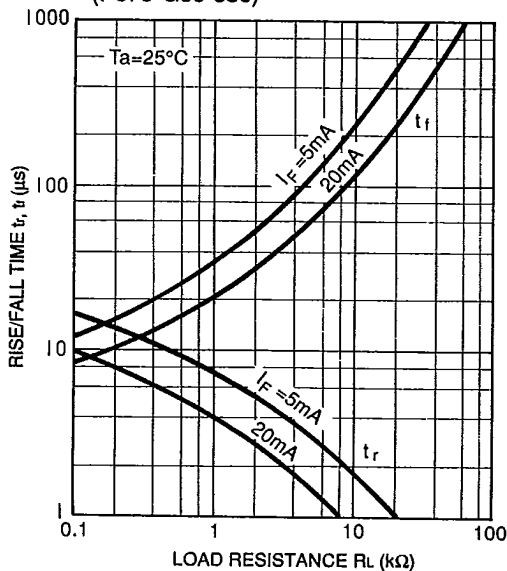
Figure 6: Rise/Fall Time vs. Load Resistance (P873-G35-380)
