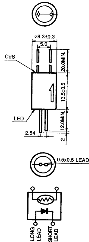
Figure 1: Dimensional Outline and Pin Connection (Unit:mm)
