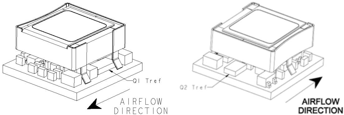
Preferred airflow direction and location of hot-spot of the module ( T_{ref} ).
