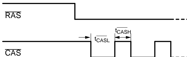
Fig. 3–13: \overline{RAS} and \overline{CAS} timing
