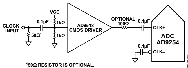
Figure 45. Single-Ended 3.3 V CMOS Sample Clock
