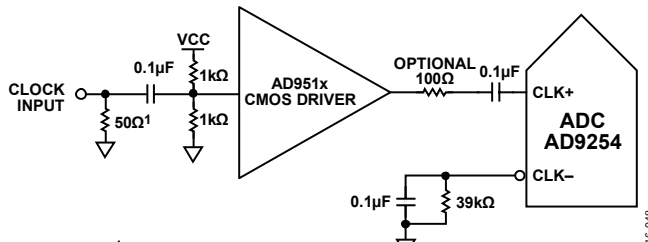
Figure 44. Single-Ended 1.8 V CMOS Sample Clock
