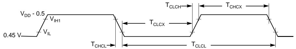
Figure 166. External Clock Waveform
