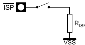
Figure 151. ISP Pull-Down Connection
