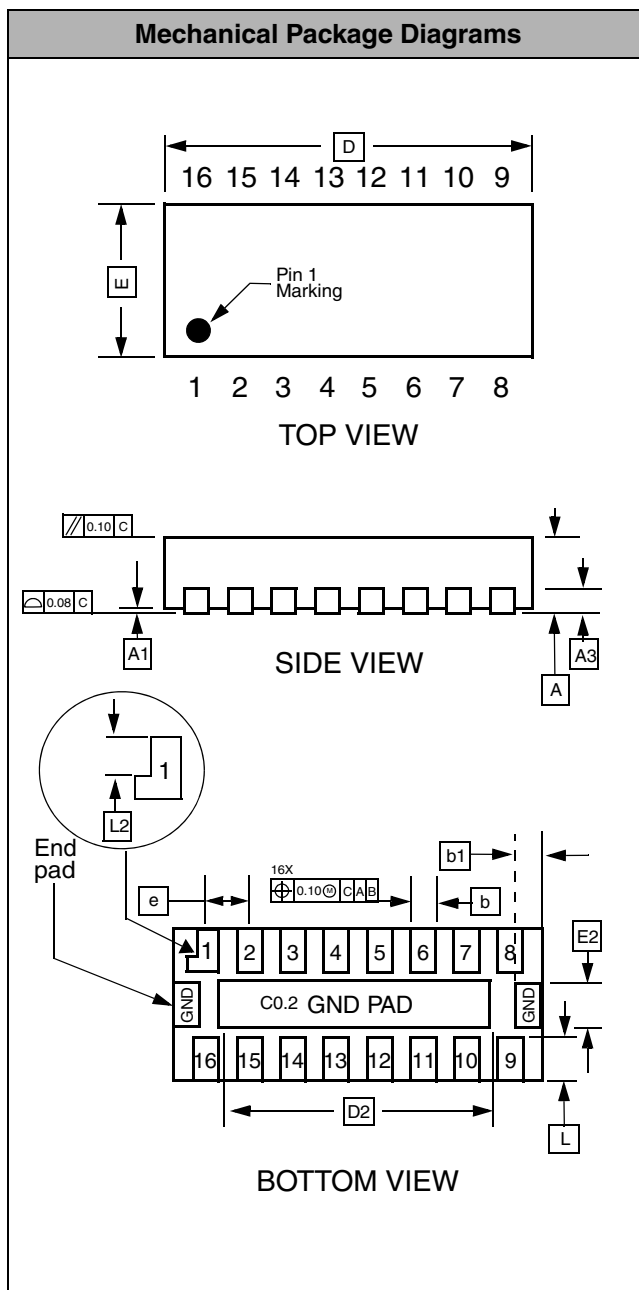
Dimensions for 16-Lead, 0.4mm pitch NuDFN package
