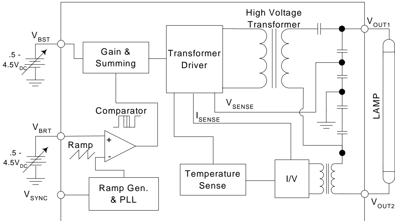
Figure 1 – RangeMAX Simplified Block Diagram
