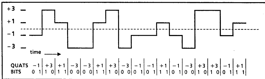
Figure 5. Example of 2B1Q Quaternary Symbols
