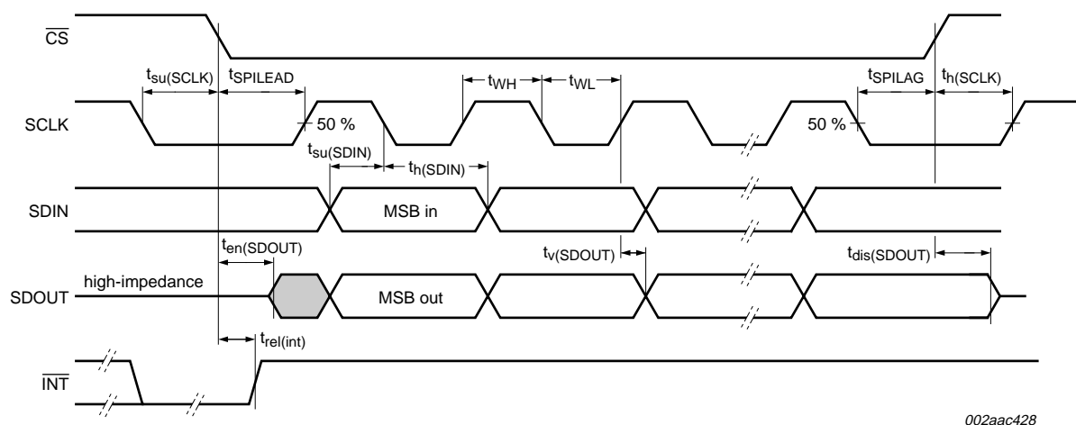
Fig 14. Timing diagram
