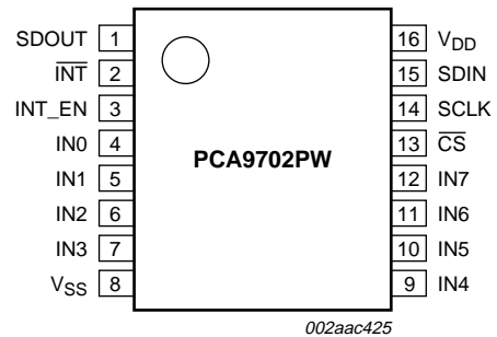
Fig 5. Pin configuration for TSSOP16
