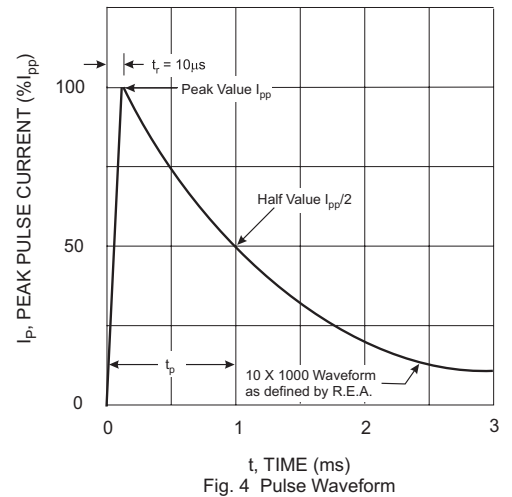
Fig. 4 Pulse Waveform
