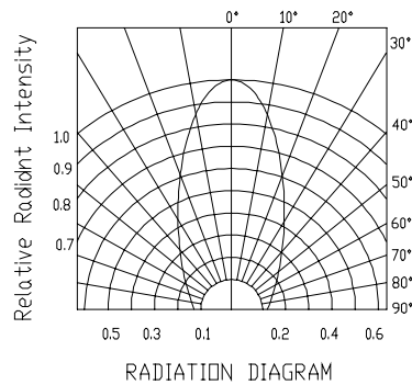
Radiation Diagram T_a=25^\circ\text{C}
