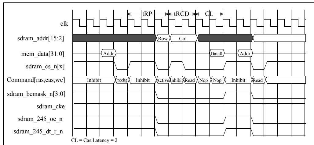
Figure 11.14 SDRAM Page-Miss Word Read
