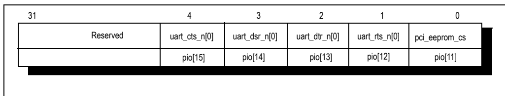
Figure 15.8 PIO Function Select Register 1 Fields
