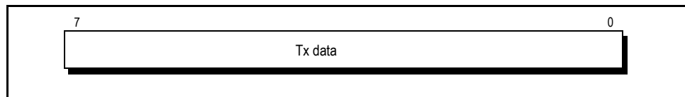
Figure 17.4 Transmit Buffer Register
