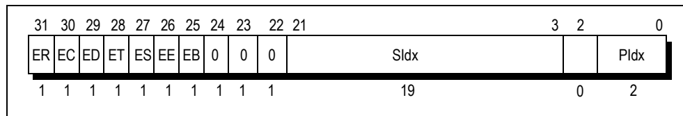
Figure 6.11 CacheErr Register
