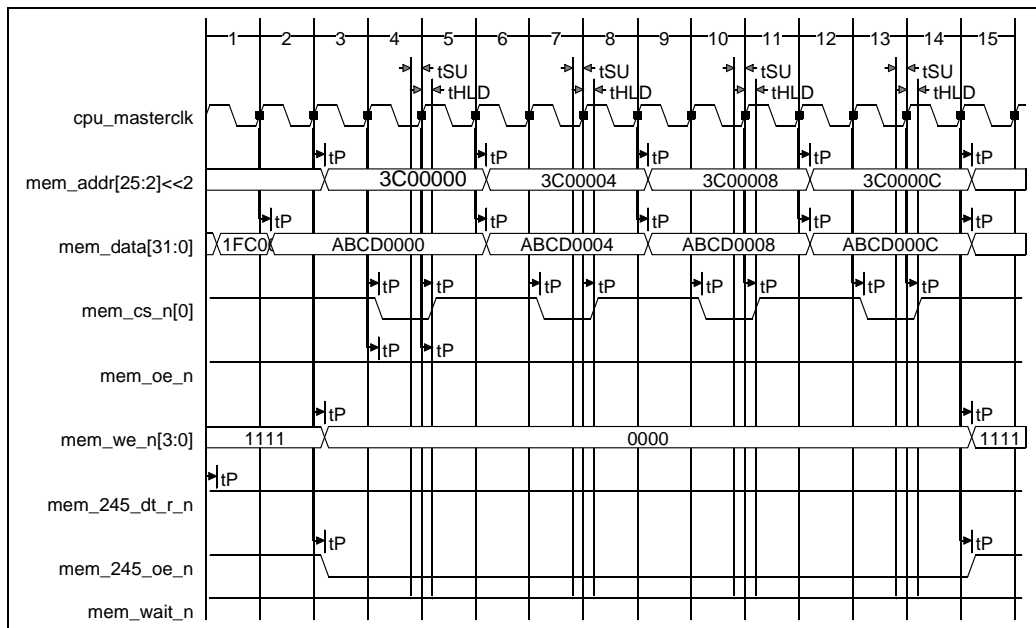
Figure 10.11 SRAM 4 Word Burst Write
