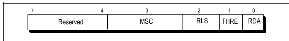
Figure 17.5 Interrupt Enable Register
