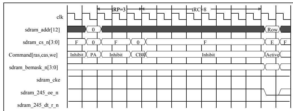
Figure 11.15 SDRAM Refresh
