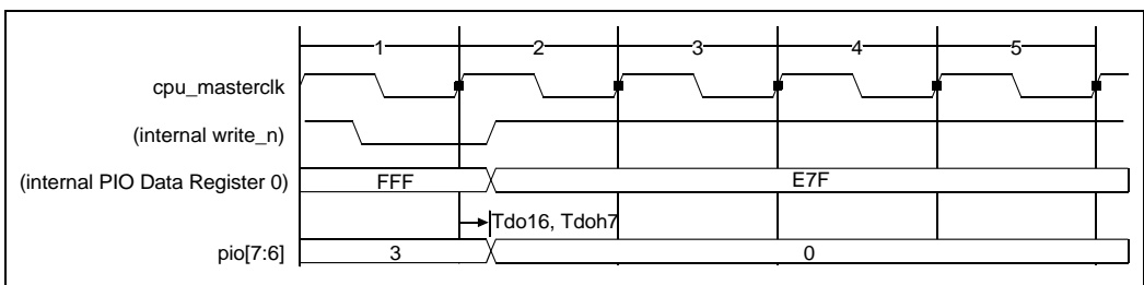
Figure 15.11 Data Register Write, Affecting PIO Output
