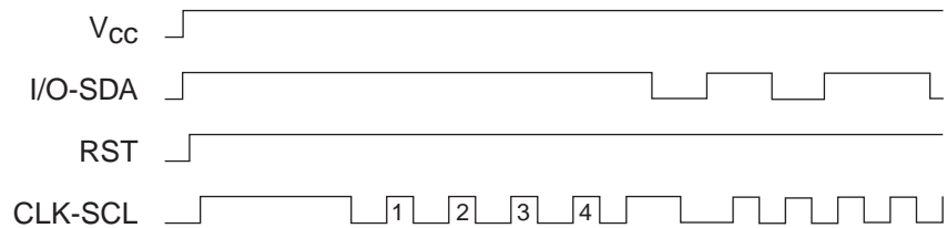
Figure 3. Synchronous Two-wire Protocol
