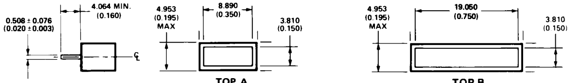
END VIEW A, B
