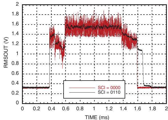
Residual Ripple for 2.6 GHz LTE Downlink @ SCI = 0110
