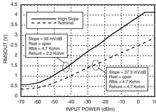
Slope Adjustment
