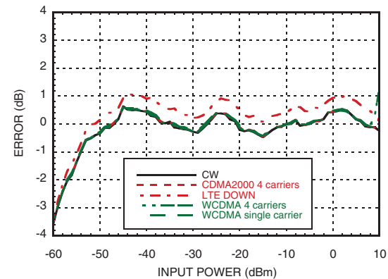
RMSOUT Error vs. Pin with Different Modulations @ 1900 MHz [2]
