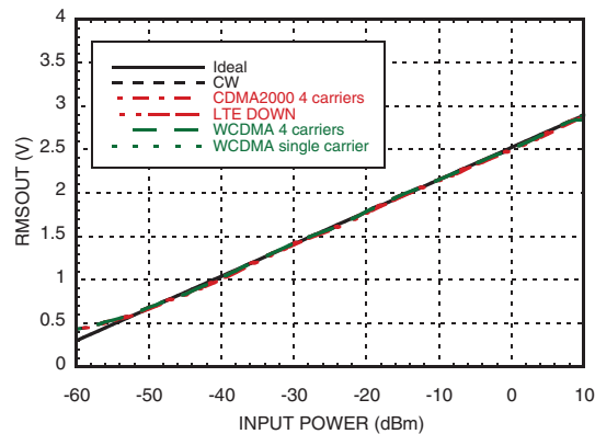
RMSOUT vs. Pin with Different Modulations @ 1900 MHz [2]
