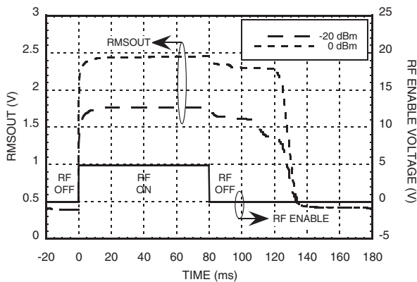
Output Response with SCI = 1111 @ 1900 MHz
