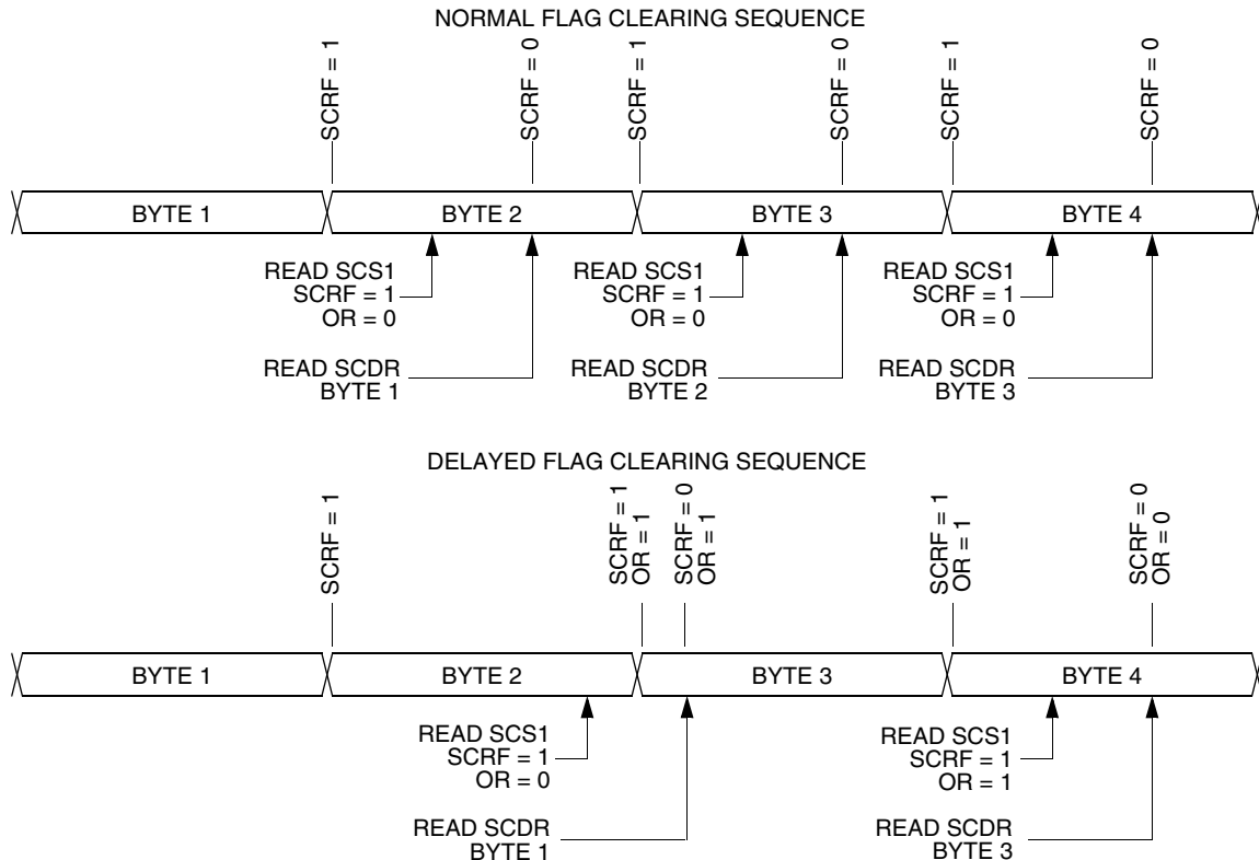
Figure 9-13. Flag Clearing Sequence
