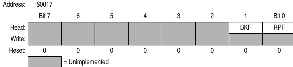
Figure 9-14. SCI Status Register 2 (SCS2)
