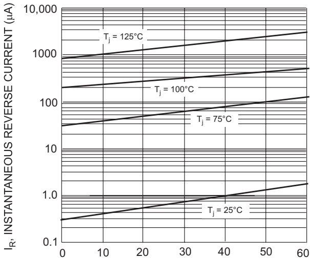
I_R , INSTANTANEOUS REVERSE CURRENT ( \mu\text{A} ) V_R , INSTANTANEOUS REVERSE VOLTAGE (V) Fig. 7 Typical Reverse Characteristics, SB550 & SB560
