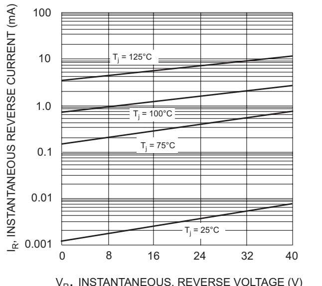
Fig. 6 Typical Reverse Characteristics, SB520 - SB540
