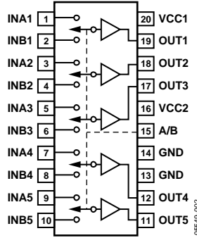
Figure 5. ADD8505 5-Channel Buffer
