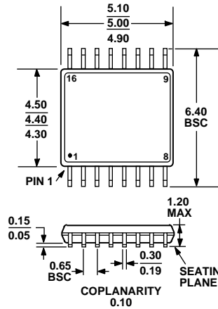
COMPLIANT TO JEDEC STANDARDS MO-153-AB Figure 13. 16-Lead Thin Shrink Small Outline Package [TSSOP] (RU-16) Dimensions shown in millimeters
