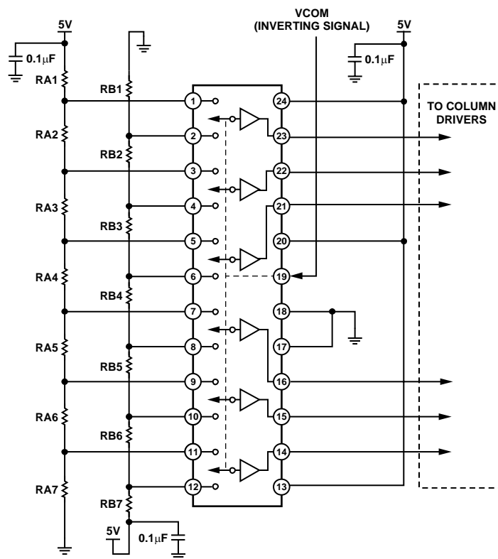
Figure 12. Typical Application
