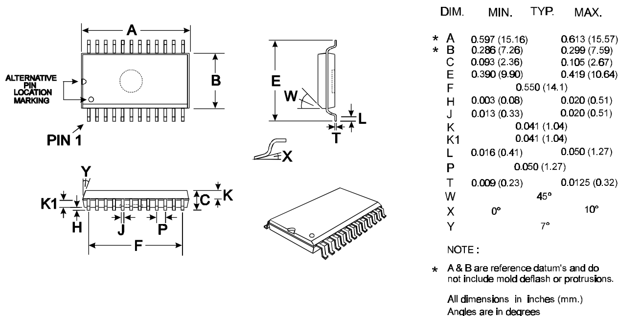
Figure 11a 24-pin SOIC (D2) Mechanical Outline: Order as part no. CMX644AD2
