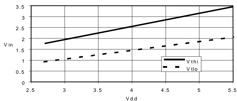
Figure 9 Typical Schmitt Trigger Input Voltage vs. V_{DD}
