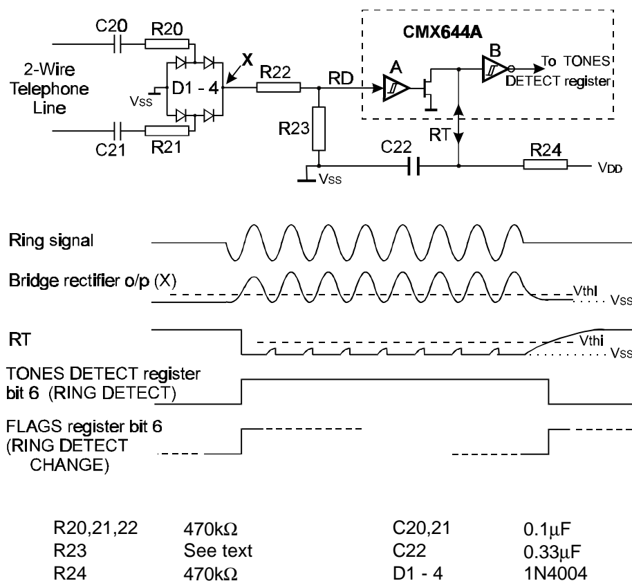
Figure 7 Ring Signal Detector Interface Circuit
