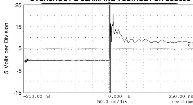
FIGURE 4 OVERSHOOT & CLAMPING VOLTAGE FOR LCD05C
