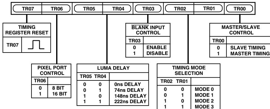
Figure 43. Timing Register 0
