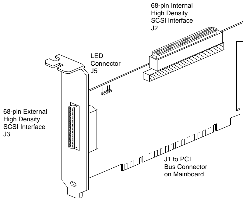
Figure 2.1 Hardware Connections for the LSI8751SP
