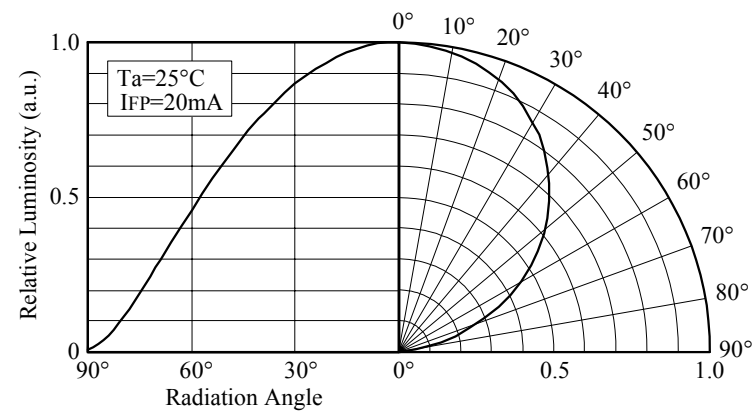
■ Directivity
