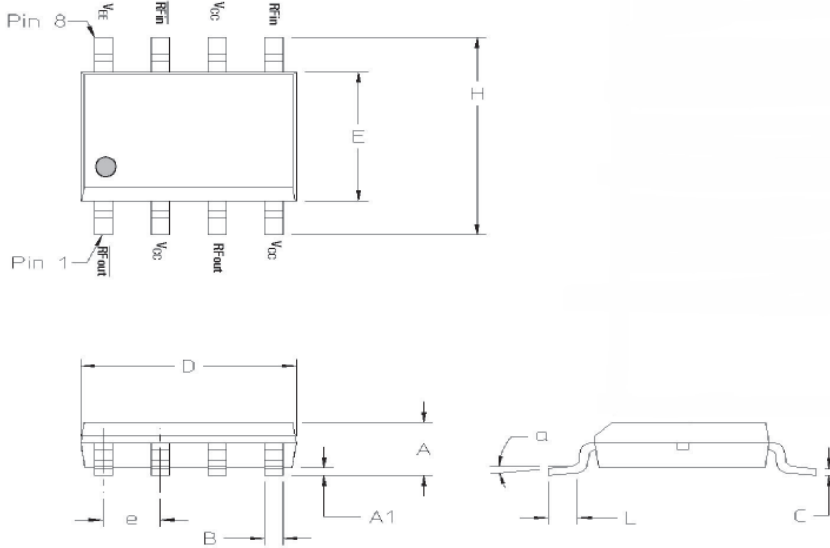
Figure 2. Package & Dimensions
